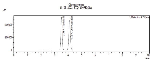
Figure 1: Simultaneous chromatogram of standard Atorvastatin & Tadalafil solution of 100 µg/ml and 100 µg/ml.
