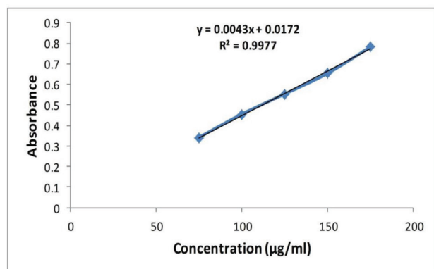
Figure 2: Standard plot for total phenol content.
