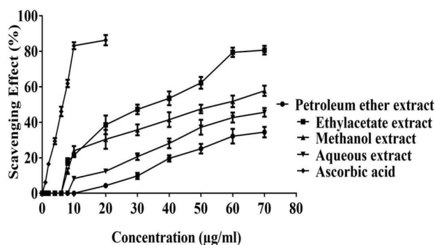
Figure 3: DPPH scavenging effects of extracts.
