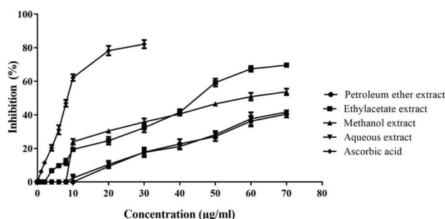
Figure 5: Nitric oxide inhibitory effects of extracts
