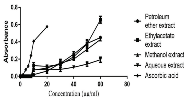
Figure 4: Ferric reducing potential of extracts.
