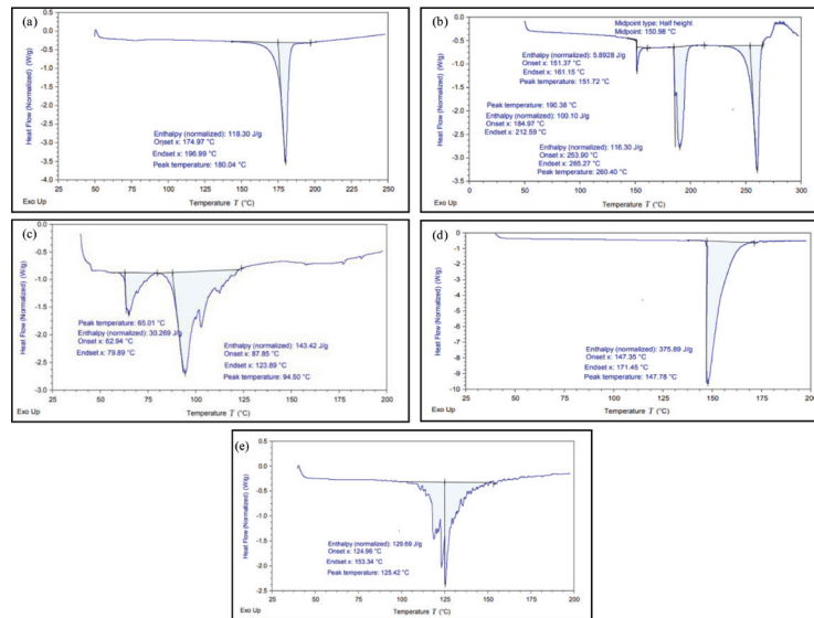
Figure 2: Differential scanning calorimetry (DSC) thermograms of (a) Curcumin showing an endothermic peak at 180.04 °C, (b) Hesperidin with an endothermic peak within the 258–262 °C range, (c) Aegle marmelos methanolic extract showing a melting point at 94.50 °C, (d) Solanum nigrum extract with a melting point at 147.78 °C, and (e) Silybum marianum extract showing a melting point at 125.42 °C.
